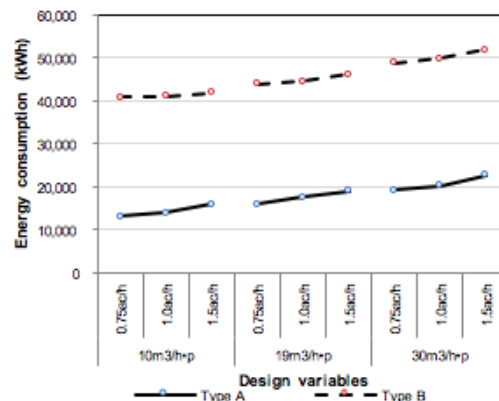
Figure 12: Annual energy demand of corridor space for different ventilation and infiltration
